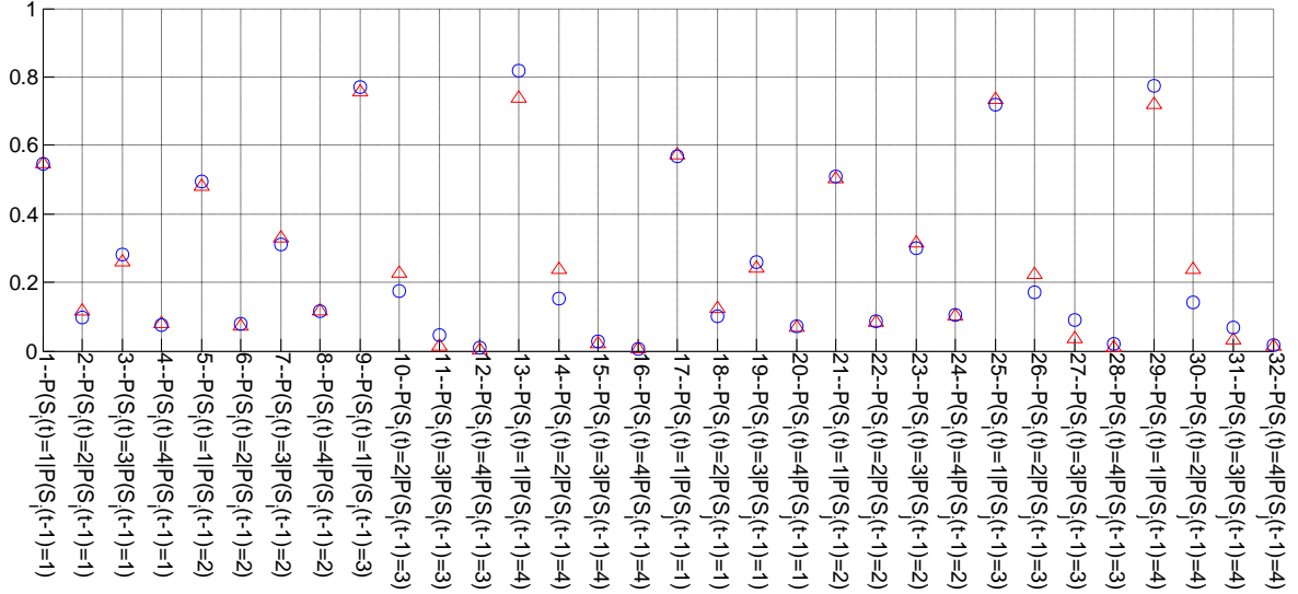
Fig. 2. Mean values of features for both classes. Triangles for pS and circles for S. Each feature has an identification number followed by its meaning. P(S_i(t) = A|S_j(t-1) = B) indicate the probability of speaker S_i to be in state A after that speaker S_j was in state B at time t-1 . The meaning of the states is: 1 = short silence, 2 = long silence, 3 = short speech, 4 = long speech.
